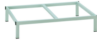
TKG / 2F ext. 607 x 815 x H 160 mm
