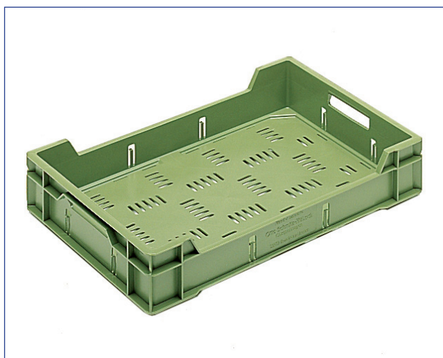
Ref. V-6410-11 - 12 lit. - 1.180 gr. ext. 600 x 400 x 65/110 mm int. 565 x 365 x 60/105 mm
