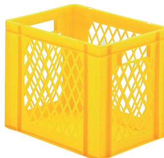
TK 400 / 320-1 ext. 400 x 300 x 320 mm int. 356 x 255 x 305 mm
